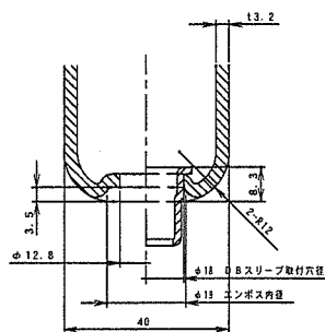
断面D-D (S=1/2)
