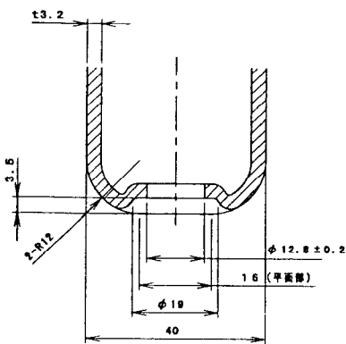
断面E-E (3カ所) (S=2/3)
