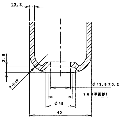
断面E-E (4カ所) (S=2/3)
