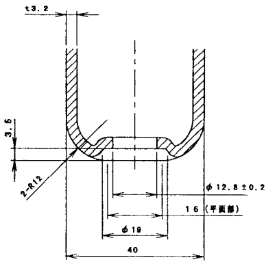
断面E-E (4力所) (S=2/3)
